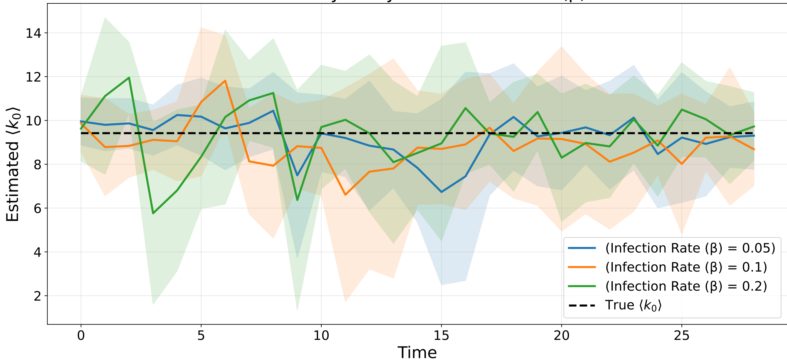
Sensitivity Analysis: Infection Rate ( \beta )
